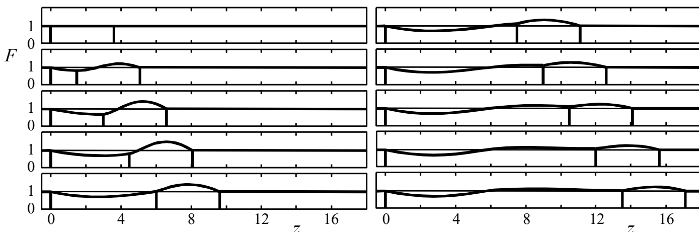
Fig. 5. Sequence of shapes during the floating zone processing of a silicon rod, obtained by non-linear numerical simulation: 1, crystal; 2, melt; 3, feed rod. The length of the molten bridge is \Lambda_0=1.8 assumed maintained constant by a suitable heating law.
