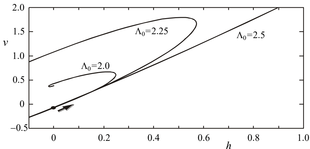
Fig. 2. Analytical results for the floating zone process of silicon crystal growth for three initial lengths of the melt ( \Lambda_0 , kept constant), showing the excess volume, v (relative to that of a cylinder) versus the relative difference in radii at both ends of the liquid, h , as the zoning progress (starting at h=0 and v=-0.08 , black point) in the direction of the arrow.
