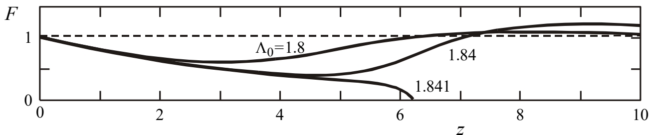
Fig. 4. Grown crystal shape for silicon floating zone processing, obtained by non-linear numerical simulation. Non-dimensional radius, F , vs. non-dimensional axial coordinate, z , for three initial lengths of the melt, \Lambda_0 (i.e. the aspect ratio, kept constant).
