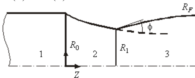
Fig. 1. Detail of growth angle geometry: 1) seed; 2) grown crystal; 3) melt.
