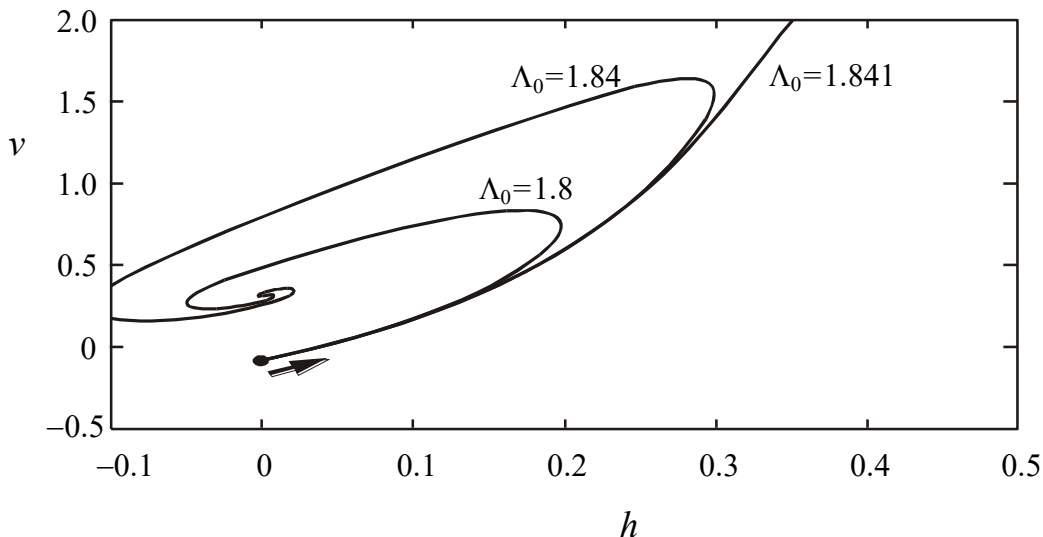
Fig. 3. Same as Figure 2 but corresponding to the non-linear numerical simulation. Note that although the start and end points are the same as in the linear analytical solution shown in Figure 2, there is not limit cycle here and the bounds on the radial deformation are nearly halved here.
