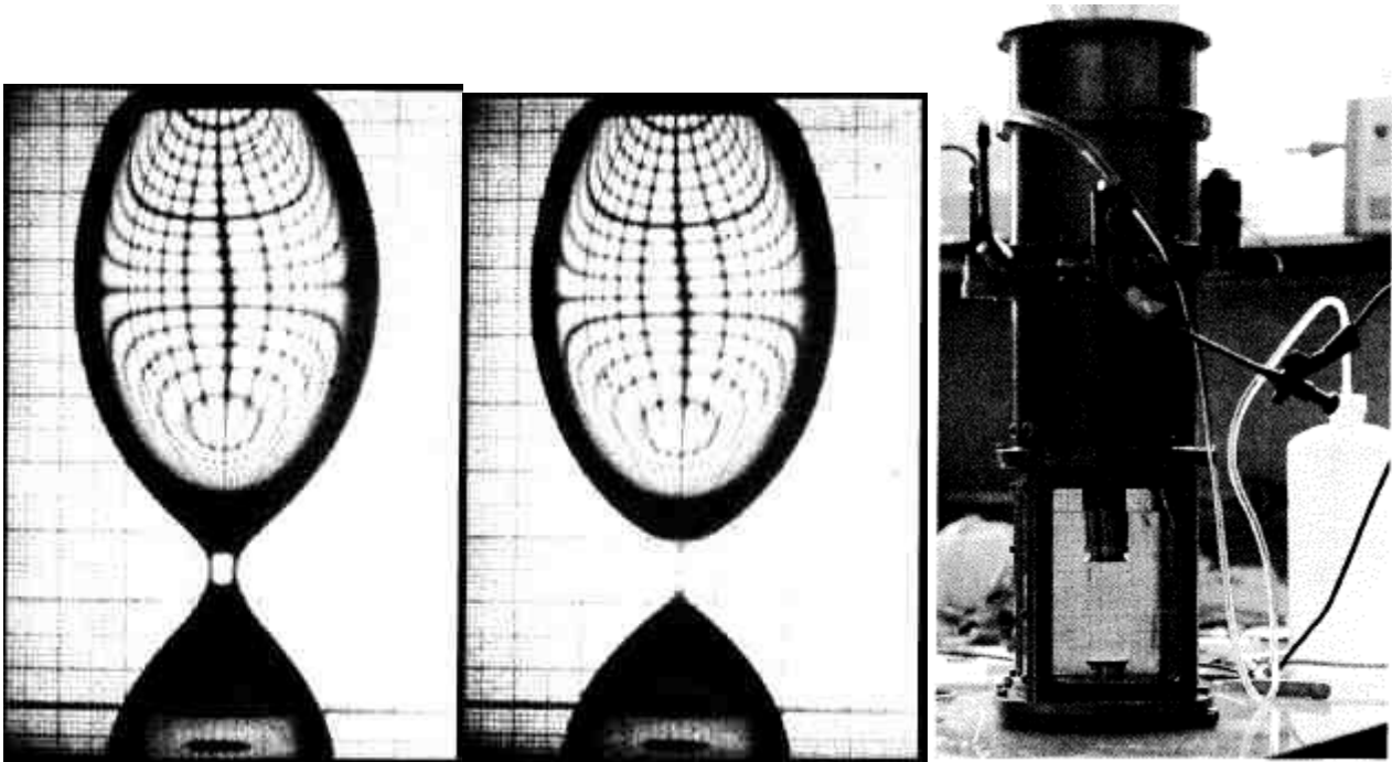
Fig. 1. Two pictures separated 0.05 s during the breakage of an 86 mm long liquid column in Texas-12 (1985), and the flight hardware been used on ground in a Plateau Tank configuration (with a liquid column formed in the test cell at the bottom). A millimetric background raster was used.
