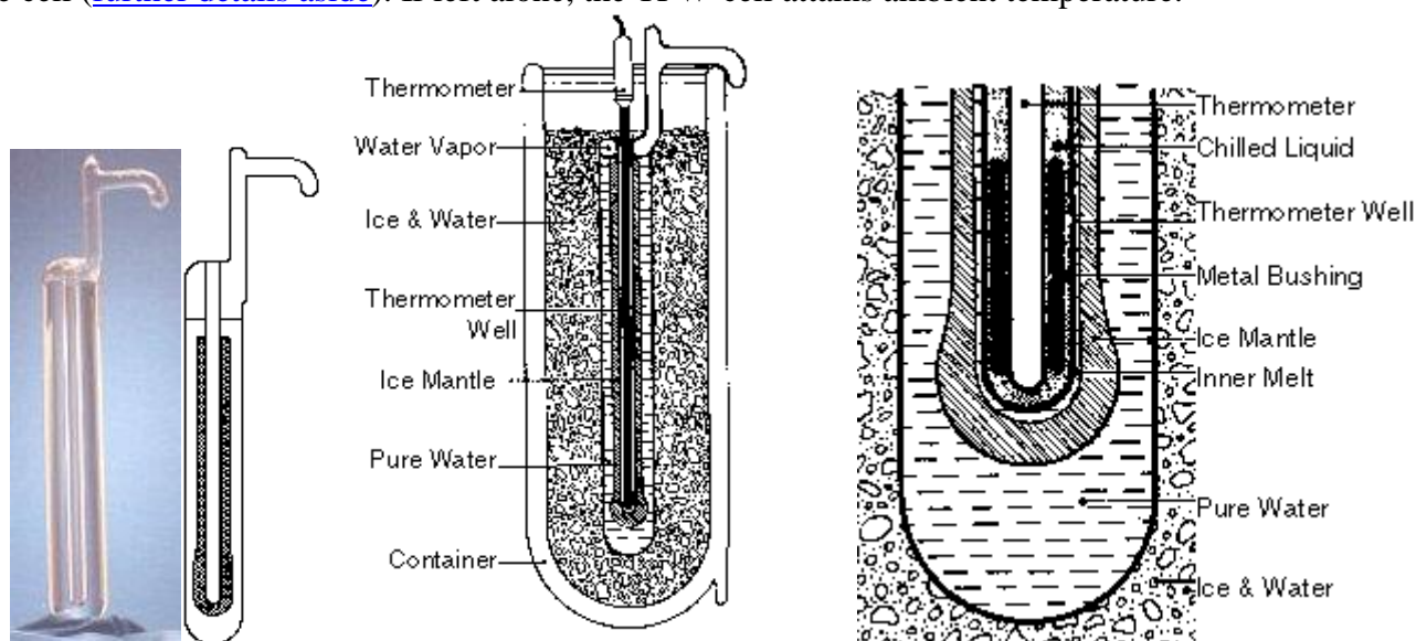
Fig. 1. Triple-point-of-water cell, with section and operational details.
