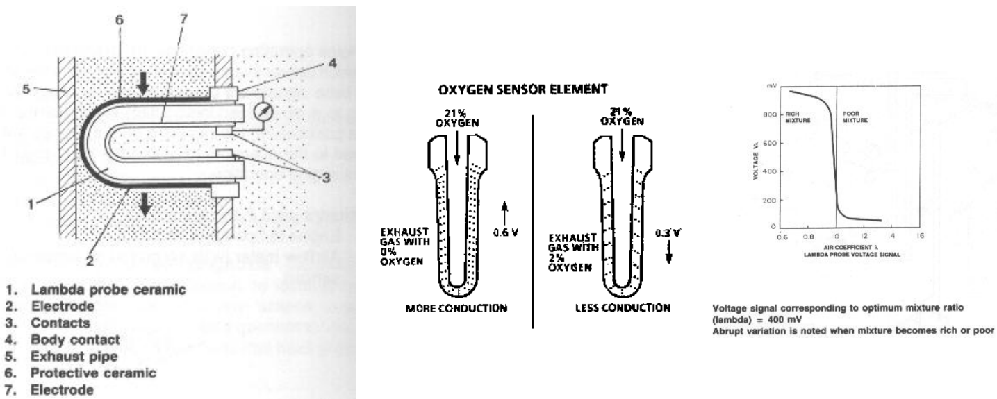
Fig. 1. Functional details of a lambda probe sensor.
