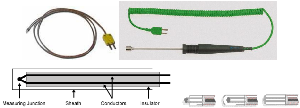
Fig. 3. Thermocouple with standard connector, surface probe with handle, internal sketch and the three different tip styles for a thermocouple.
